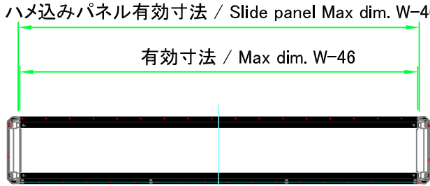
ねじ止めパネル有効寸法 / Screwed panel Max dim. W-46
